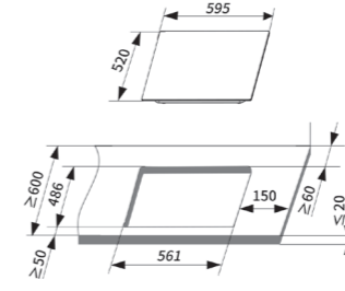
RB-H3280 IH智慧感應三口爐(橫向)
